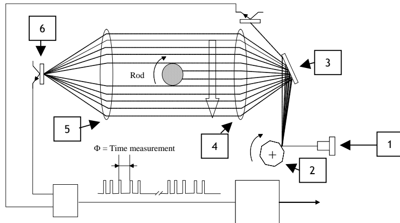
Figure 1 - Diagram of a laser gauging system
